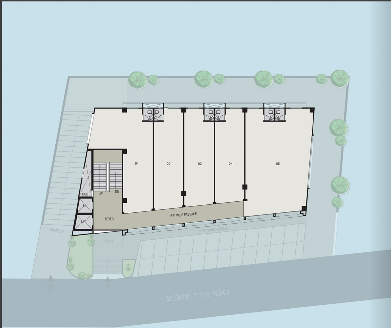
2 nd to 5 th Floor Plan
